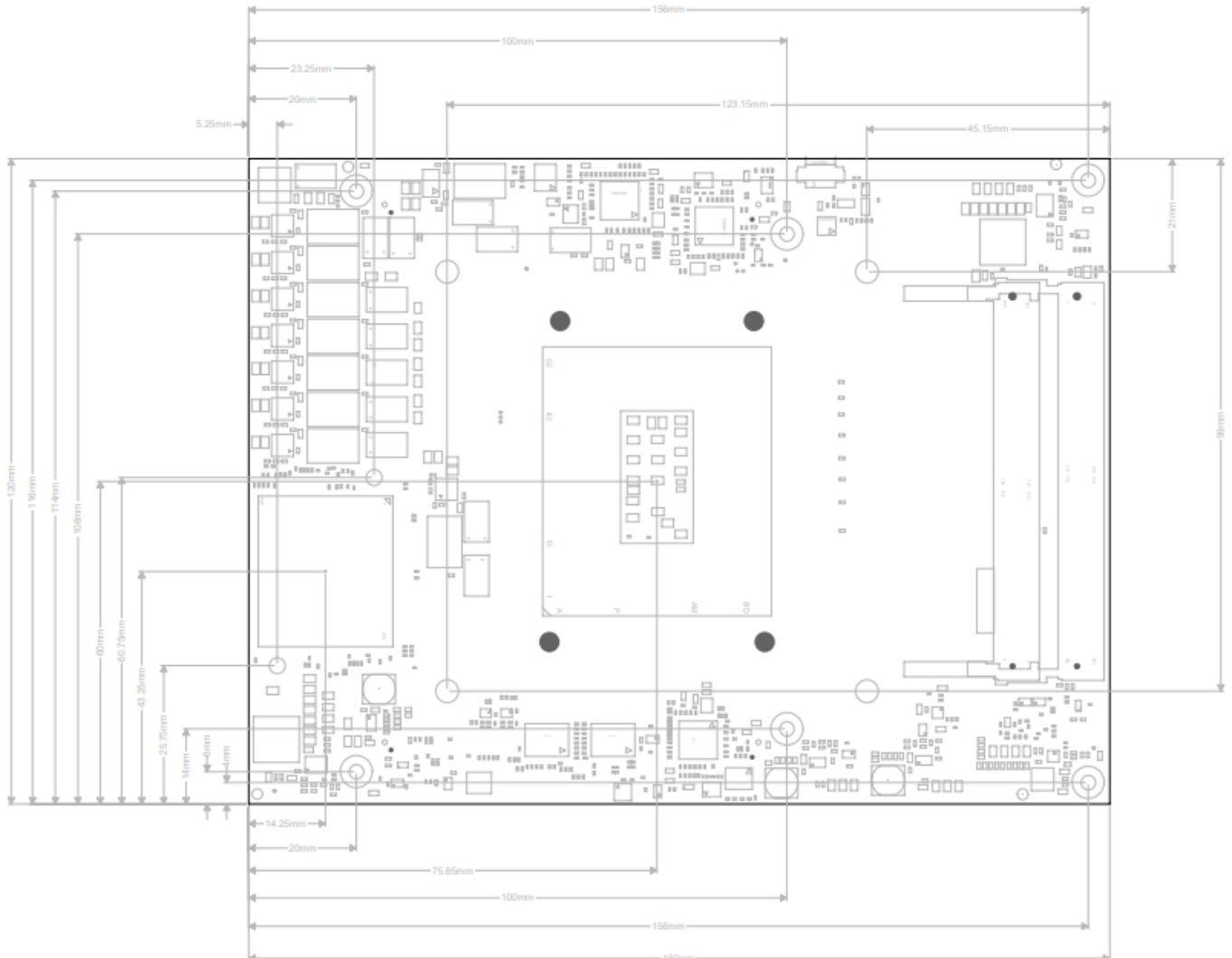
Figure 6: Module Dimensions
