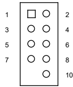
Figure 16: USB 2.0 Port 4, 5 Pin Header CN20, Port 6, 7 Pin Header CN21
