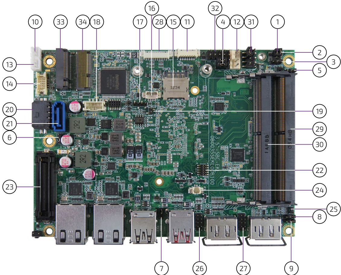
Figure 2: Top Side
