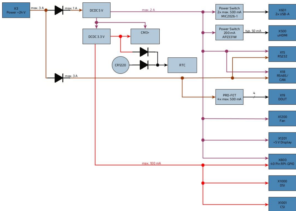
Figure 3: Power Tree
