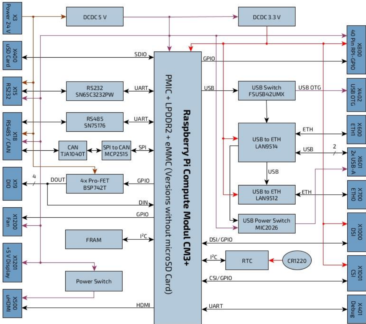
Figure 4: Block Diagram
