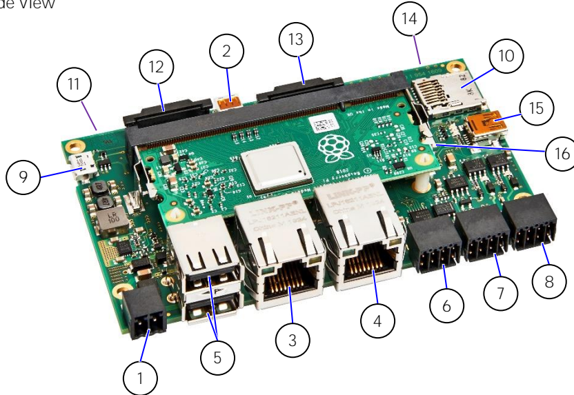
Figure 5: Top Side View
