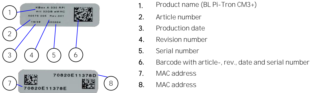
Figure 8: BL Pi-Tron CM3+ Type Label (Example)
